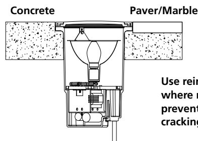
DB8 In Concrete With Trim Ring
